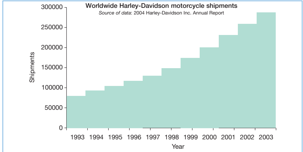
Figure 12.5 Histogram
