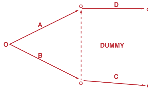
FIGURE 12–5. Dummy activity.
