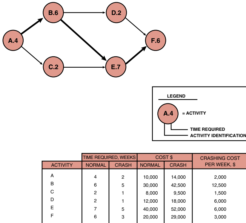
FIGURE 12-16. CPM network.
