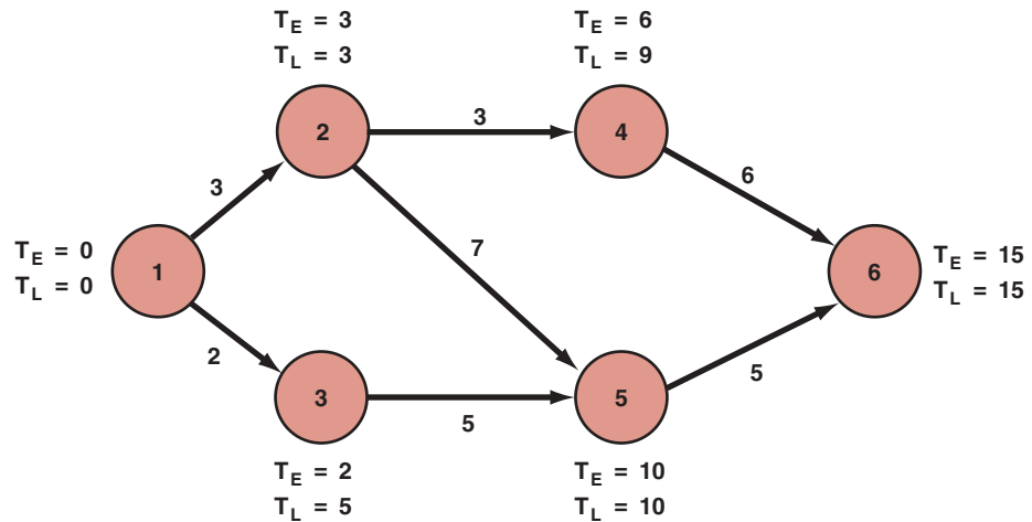
FIGURE 12-6. PERT network with slack time.
