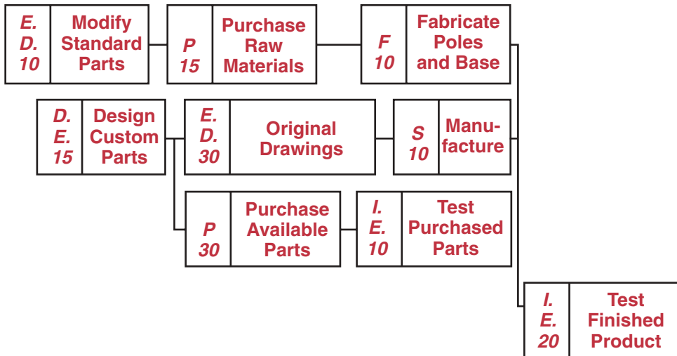
FIGURE 22-5. Resource-leveled project.
