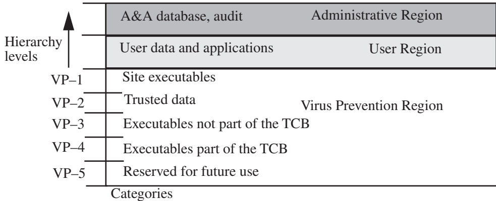
Figure 5-3 The three MAC regions in the MAC lattice (modified from the DG/UX Security Manual [230], p. 4-7, Figure 4-4). TCB stands for “trusted computing base.”
