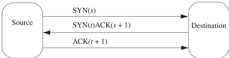
Figure 21–2 The TCP three-way handshake. The SYN packet is a TCP packet with sequence number s (or t ) and the SYN flag set. Likewise, the ACK packet is a TCP packet with acknowledgment number s + 1 (or t + 1 ) and the ACK flag set. The middle message is a single TCP packet with both SYN and ACK flags set.
