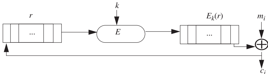
Figure 10–1 Diagram of cipher feedback mode. The register r is enciphered with key k and algorithm E . The rightmost bit of the result is exclusive-or'ed with one bit of the plaintext m_i to produce the ciphertext bit c_i . The register r is right shifted one bit, and c_i is fed back into the leftmost bit of r .
