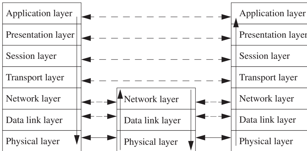
Figure 10–2 The ISO/OSI model. The dashed arrows indicate peer-to-peer communication. For example, the transport layers are communicating with each other. The solid arrows indicate the actual flow of bits. For example, the transport layer invokes network layer routines on the local host, which invoke data link layer routines, which put the bits onto the network. The physical layer passes the bits to the next “hop,” or host, on the path. When the message reaches the destination, it is passed up to the appropriate level.
