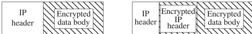
Figure 10–4 The packet on the left is in transport mode, because the body of the packet is encrypted but its header is not. The packet on the right is in tunnel mode, because the packet header and the packet body are both encrypted. The unencrypted IP header is used to deliver the encrypted packet to a system on which it can be decrypted and forwarded.
