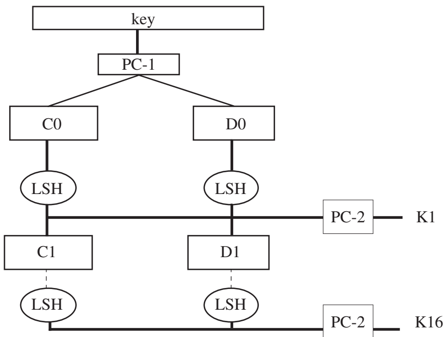
Figure 8–5 DES key schedule generation. PC-1 and PC-2 are permutation tables; LSH is a table of left shifts (rotations).
