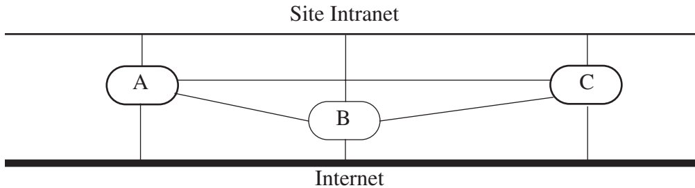
Figure 22–3 Site with three firewalls, each of which has an intrusion detection system running the IDIP protocol.
