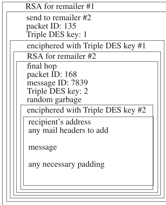
Figure 13–2 A Mixmaster message. This is a fragment of a multipart message sent through two remailers. Messages are enciphered using both RSA and Triple DES, and random garbage is added as well as padding. The recipient's address is visible only to the last remailer.
