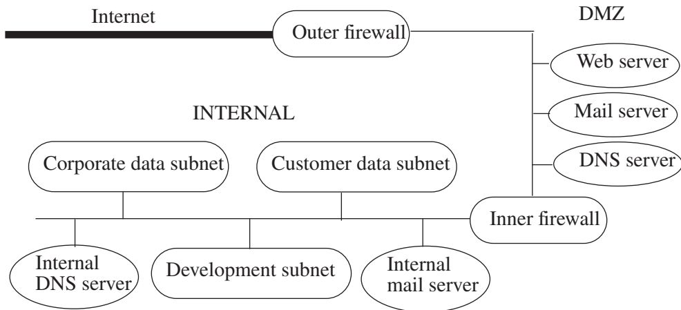
Figure 23–1 The network designed for the Dribble Corporation. The “outer firewall” sits between the Internet and the company network. The subnet labeled “DMZ” provides limited public access to various servers. The “inner firewall” sits between the DMZ and the subnets that are not to be accessed by the public. These subnets share common mail and DNS servers that, like the other hosts, are not publicly accessible.
