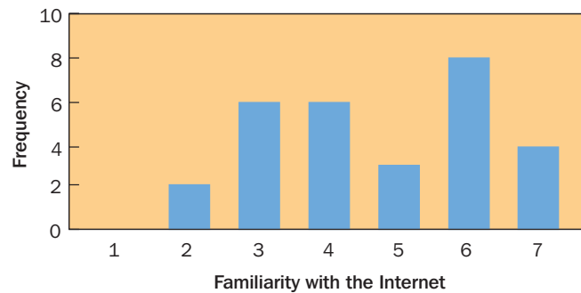
Figure 18.1 Frequency histogram
