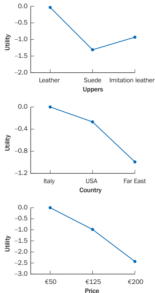
Figure 24.10 Part-worth functions
